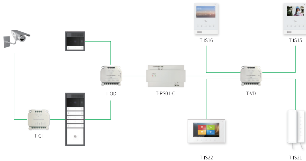
Star Connection:
