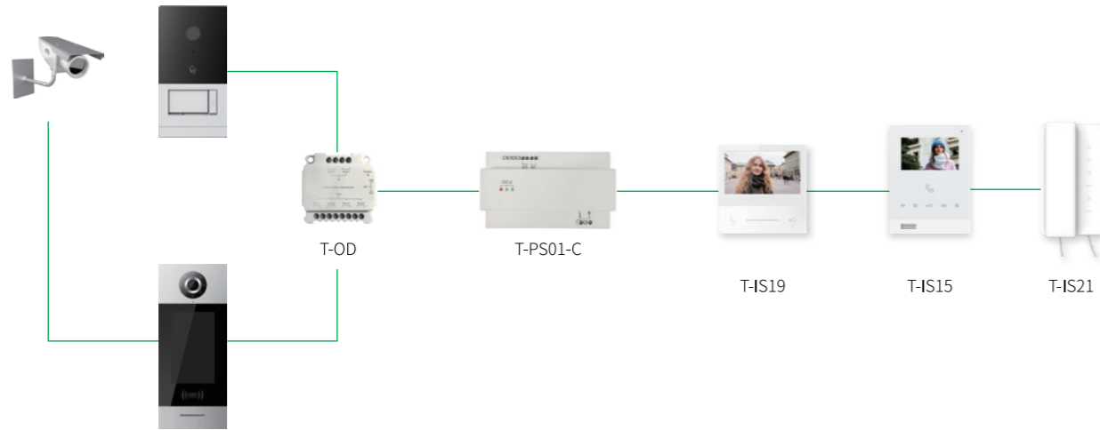
Daisy-chain Connection:
